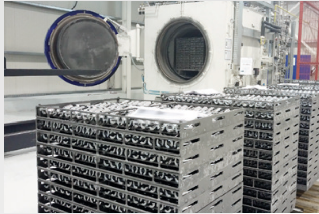
Hardening - gas nitriding
